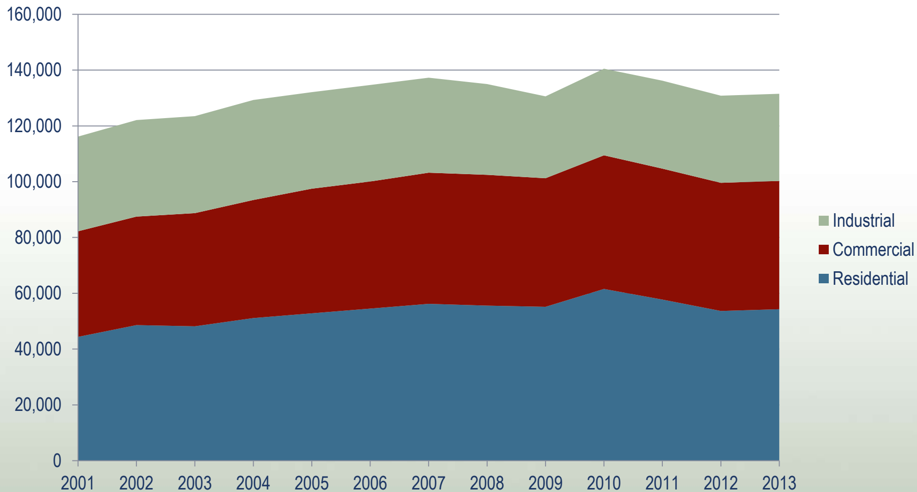
Retail Sales of Electricity in Georgia, million kWh
