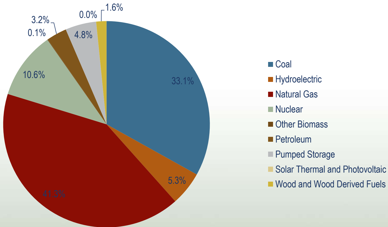
Electric Capacity by Fuel, 2012
