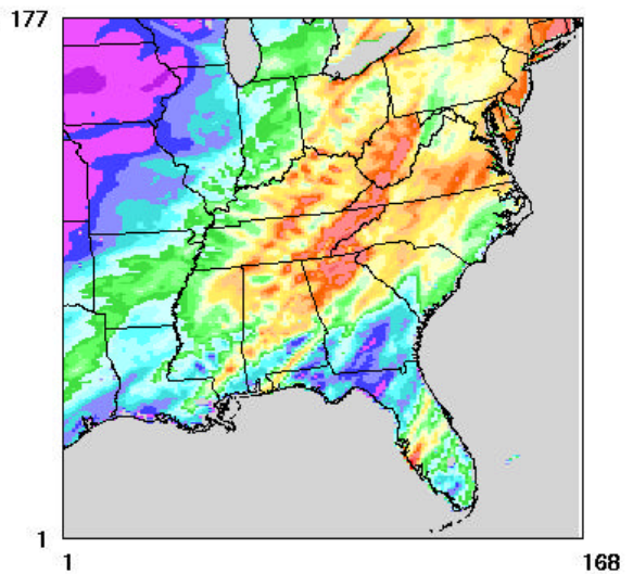
Figure 91. The November 2002 12-km accumulated precipitation from the Climate Prediction Center is juxtaposed with the MM5 accumulated precipitation.
