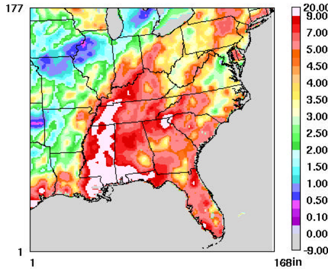
Figure 89. The September 2002 12-km accumulated precipitation from the Climate Prediction Center is juxtaposed with the MM5 accumulated precipitation.
