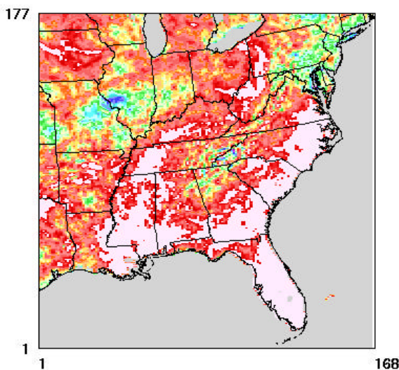
Figure 87. The July 2002 12-km accumulated precipitation from the Climate Prediction Center is juxtaposed with the MM5 accumulated precipitation.
