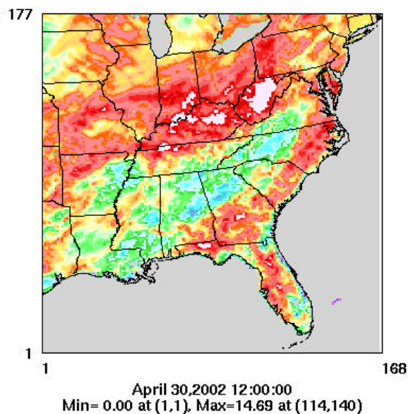
Figure 84. The April 2002 12-km accumulated precipitation from the Climate Prediction Center is juxtaposed with the MM5 accumulated precipitation.
