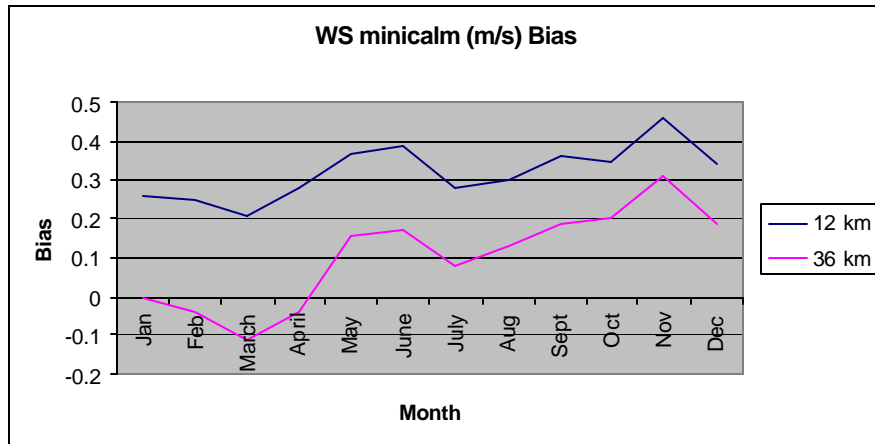
Figure 61. VISTAS region wind speed (minimum calms) biases (m/s) are plotted for both 12-km and 36-km resolutions.
