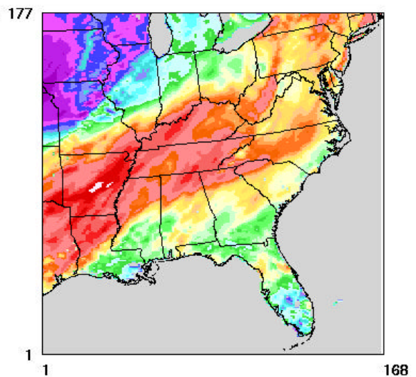
Figure 92. The December 2002 12-km accumulated precipitation from the Climate Prediction Center is juxtaposed with the MM5 accumulated precipitation.
