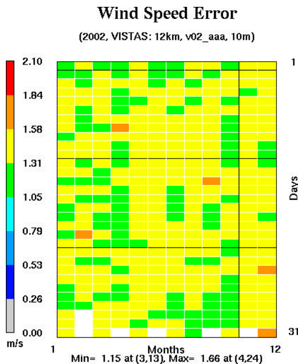
Figure 54. The 2002 12-km VISTAS “Bakergram” for wind speed (regular) error is plotted. The data are shown in a calendar-like layout so that the bias on the first day of January.
