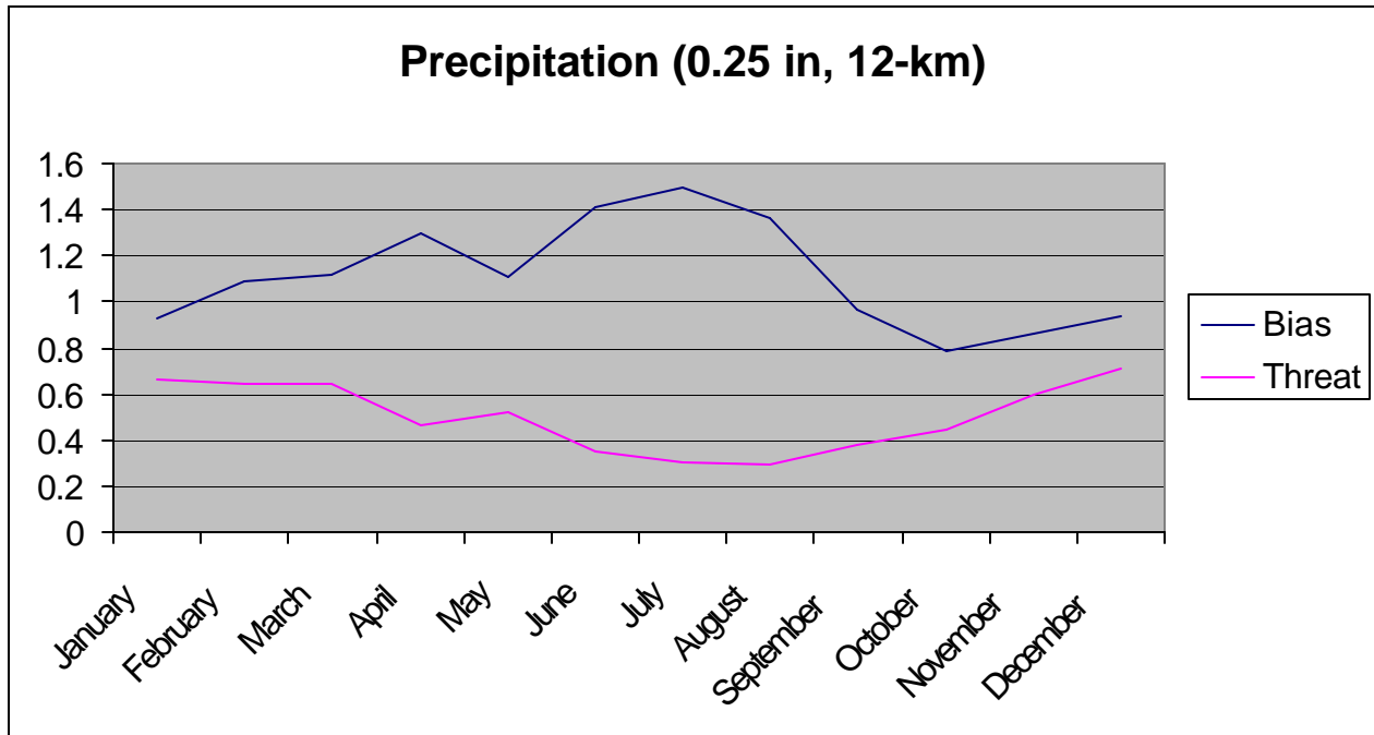
Figure 97. The 0.25 in threshold precipitation bias and threat score for the 12-km domain is shown for modeling year 2002.
