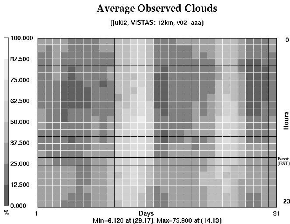
Figure 75. The July 2002 12-km VISTAS “Bakergram” for observed cloud coverage (%) is plotted. The hourly values are shown in a calendar-like layout so that the upper left cell represents the 00Z bias on the first day.
