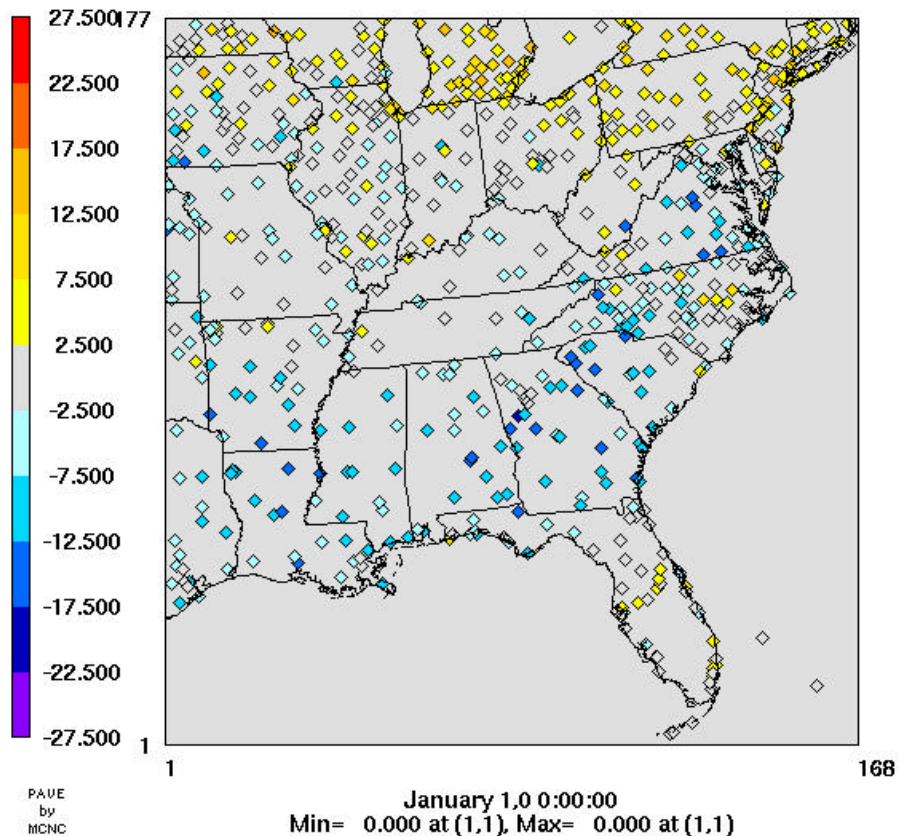
Figure 40. Site-specific RH biases (%) for November 2002 are displayed for each site in the 12-km grid. Note that the PAVE date label (January 1, 0) is nonsensical and should be ignored since it is only a placeholder.
