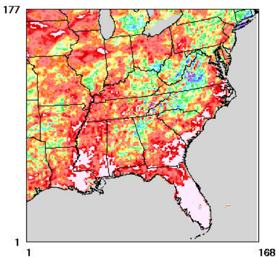
Figure 88. The August 2002 12-km accumulated precipitation from the Climate Prediction Center is juxtaposed with the MM5 accumulated precipitation.
