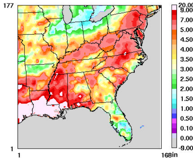
Figure 90. The October 2002 12-km accumulated precipitation from the Climate Prediction Center is juxtaposed with the MM5 accumulated precipitation.
