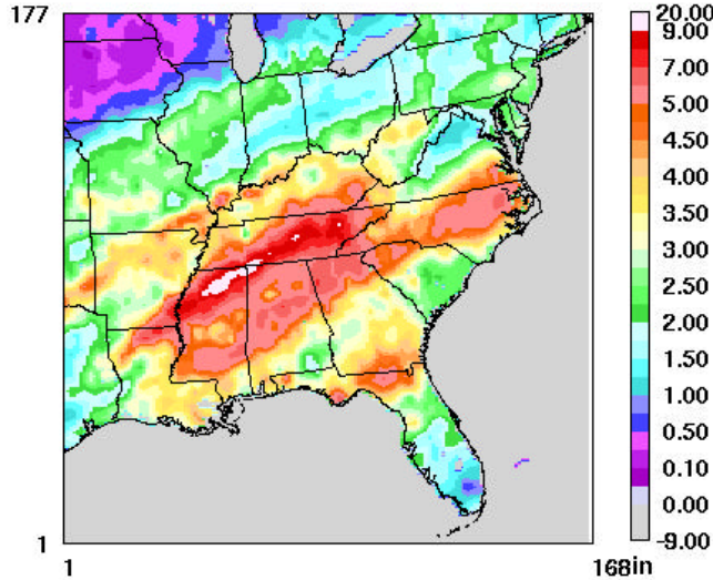
Figure 81. The January 2002 12-km accumulated precipitation from the Climate Prediction Center is juxtaposed with the MM5 accumulated precipitation.
