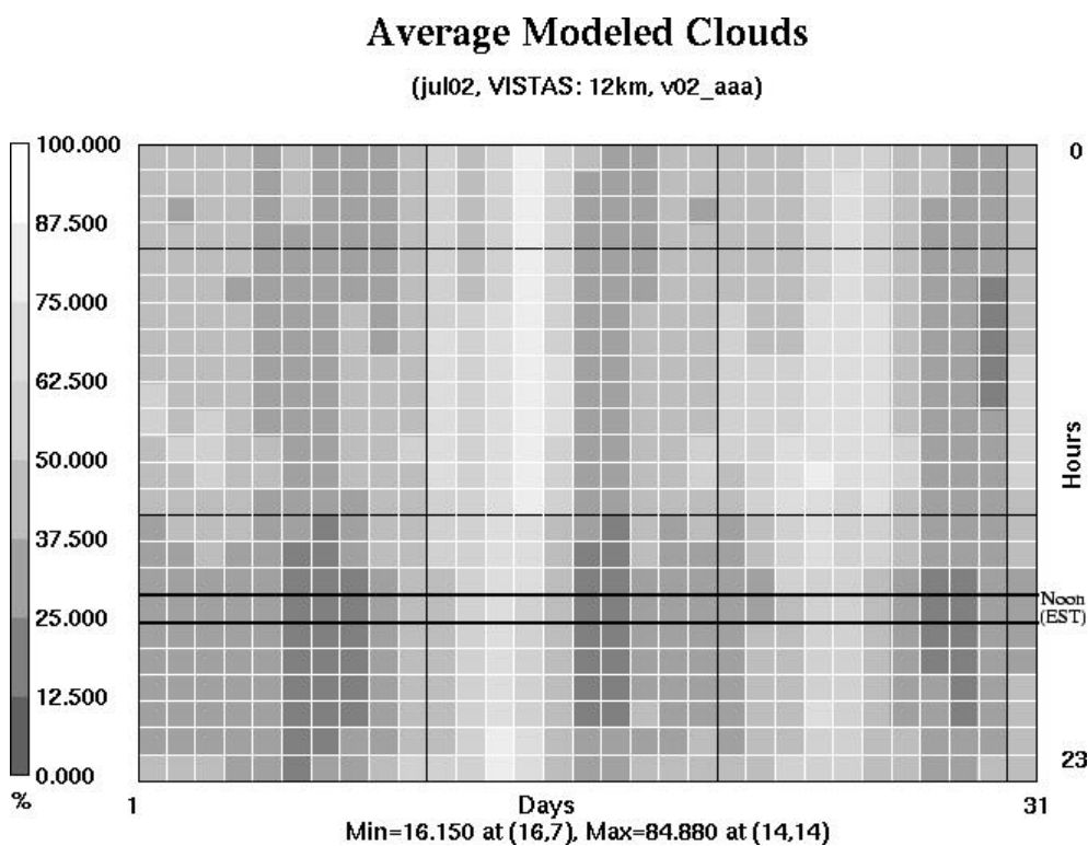
Figure 76. The July 2002 12-km VISTAS “Bakergram” for modeled cloud coverage (%) is plotted. The hourly values are shown in a calendar-like layout so that the upper left cell represents the 00Z bias on the first day.
