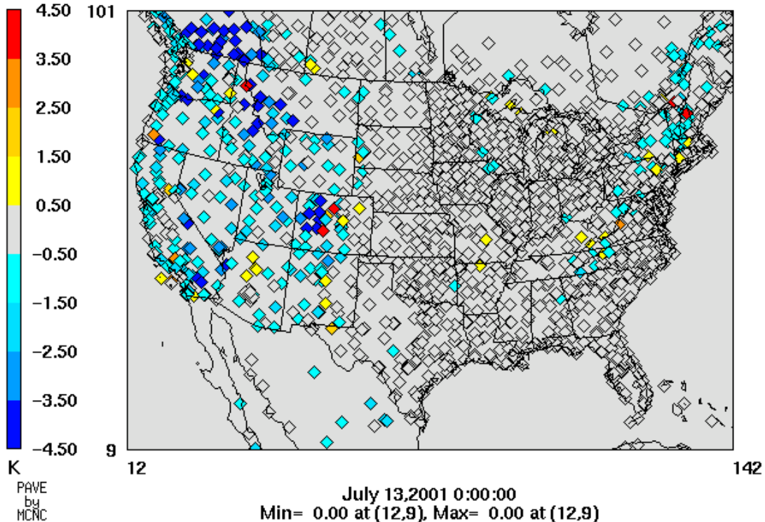
Figure 17. Model/obs elevation differences are converted to temperatures and plotted for the US portion of the 36-km grid. The temperatures are calculated assuming a standard atmosphere lapse rate of 6.5C/km, and practically indicate the temperature biases that might result solely by ignoring elevation-induced temperature effects. All of the observing sites are shown, including those sites that we ignore when calculating statistics due to their elevations being more than 500m different than the corresponding model elevations.
