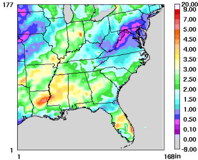
Figure 82. The February 2002 12-km accumulated precipitation from the Climate Prediction Center is juxtaposed with the MM5 accumulated precipitation.
