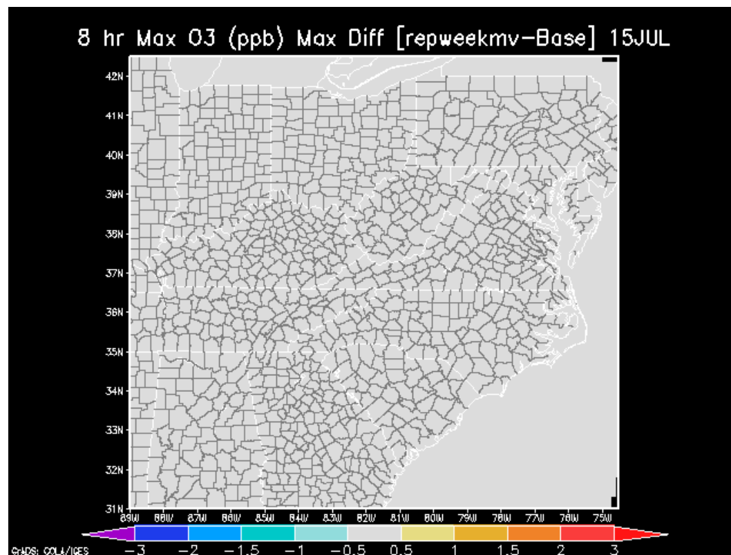
Figure 13. Absolute differences in daily 8-hour maximum ozone concentrations for July 15 th (Representative week mobile emissions versus daily mobile emissions).
