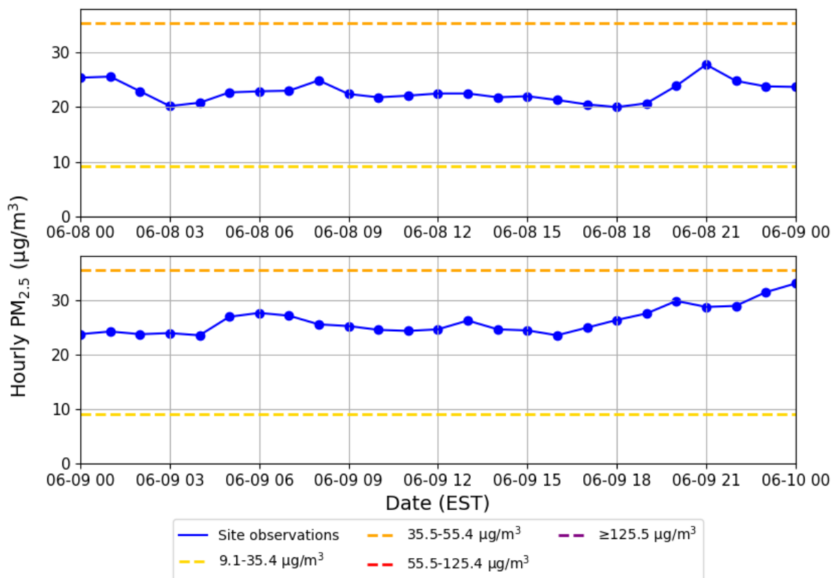
135 Figure E2. Hourly PM 2.5 concentrations at the Augusta site on June 8 and 9, 2023. The solid lines with dots show observations, and the dashed lines show AQI tiers adjusted for the 2024 PM 2.5 NAAQS.
