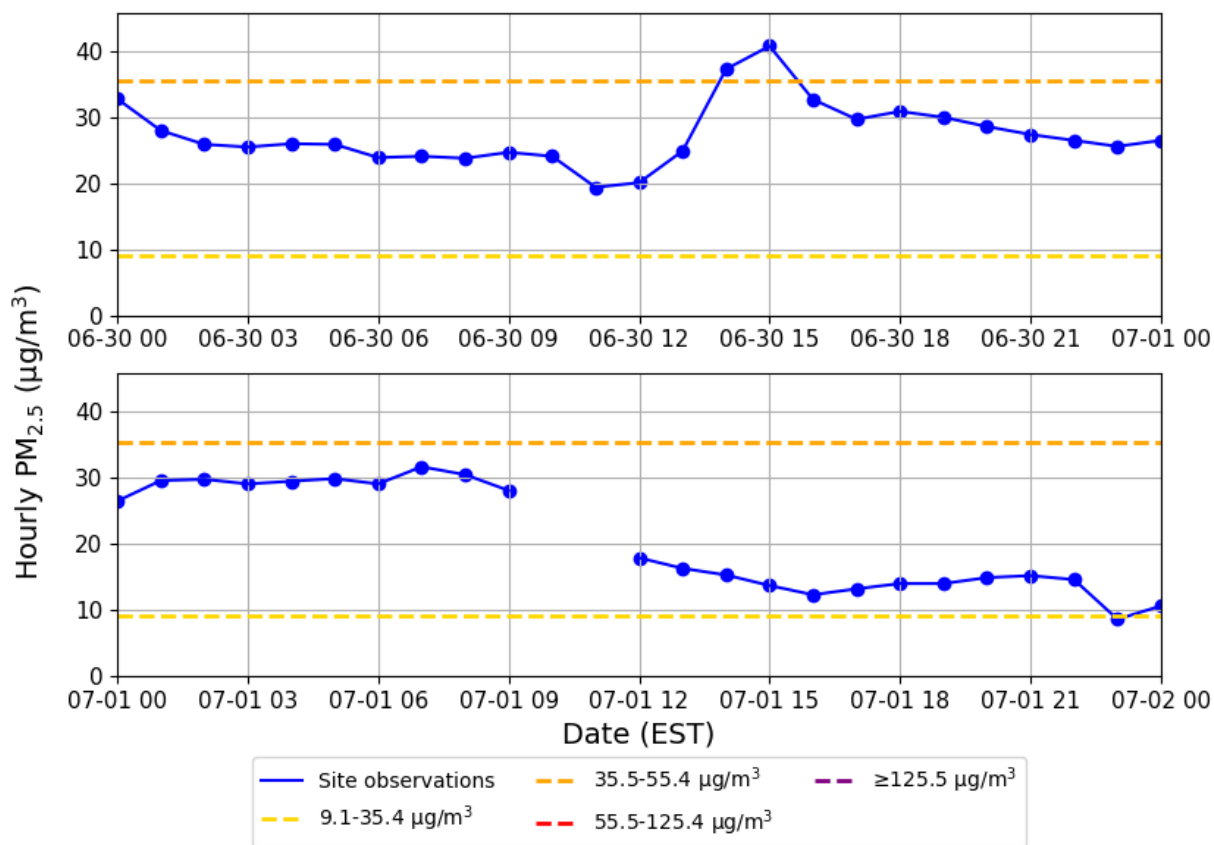
160 Figure E7. Hourly PM 2.5 concentrations at the Augusta site on June 30 and July 1, 2023. The solid lines with dots show observations, and the dashed lines show AQI tiers adjusted for the 2024 PM 2.5 NAAQS.
