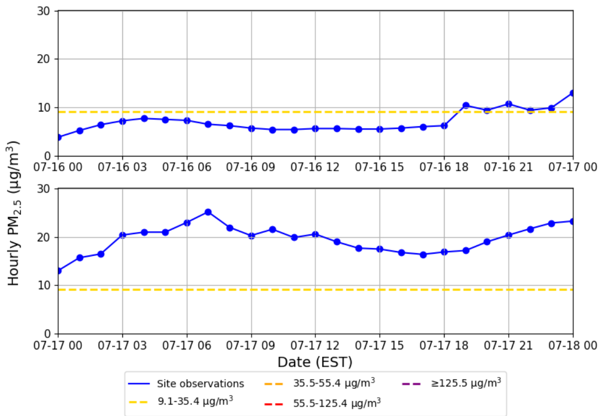
165 Figure E8. Hourly PM 2.5 concentrations at the Augusta site on July 16 and 17, 2023. The solid lines with dots show observations, and the dashed lines show AQI tiers adjusted for the 2024 PM 2.5 NAAQS.
