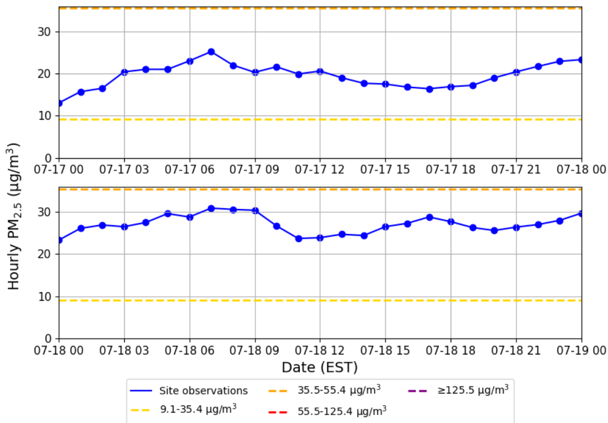
170 Figure E9. Hourly PM 2.5 concentrations at the Augusta site on July 17 and 18, 2023. The solid lines with dots show observations, and the dashed lines show AQI tiers adjusted for the 2024 PM 2.5 NAAQS.
