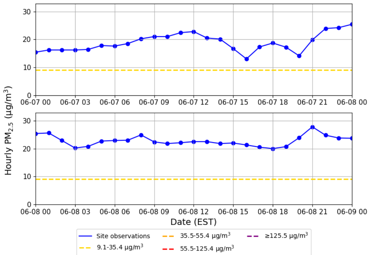
130 Figure E1. Hourly PM 2.5 concentrations at the Augusta site on June 7 and 8, 2023. The solid lines with dots show observations, and the dashed lines show AQI tiers adjusted for the 2024 PM 2.5 NAAQS.
