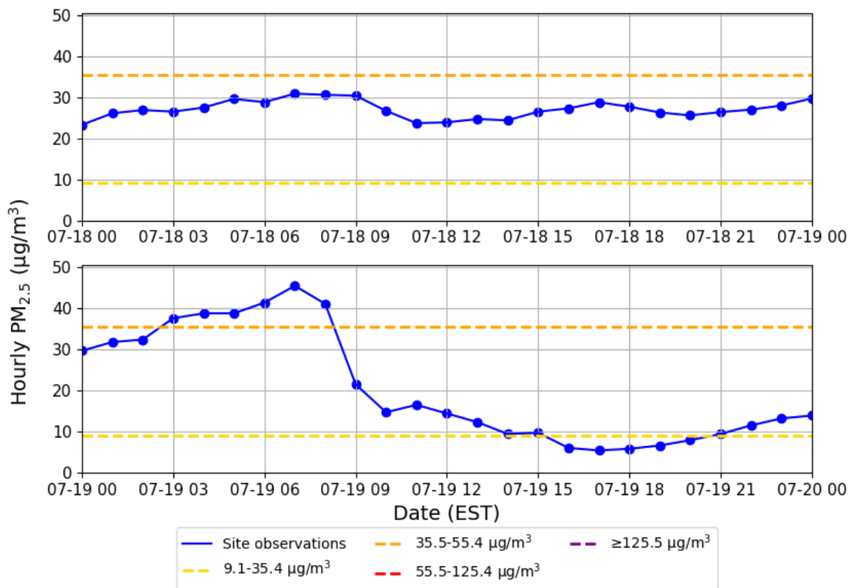
175 Figure E10. Hourly PM 2.5 concentrations at the Augusta site on July 18 and 19, 2023. The solid lines with dots show observations, and the dashed lines show AQI tiers adjusted for the 2024 PM 2.5 NAAQS.
