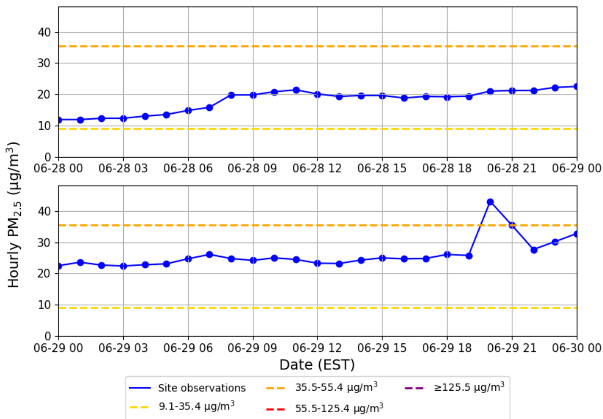
150 Figure E5. Hourly PM 2.5 concentrations at the Augusta site on June 28 and 29, 2023. The solid lines with dots show observations, and the dashed lines show AQI tiers adjusted for the 2024 PM 2.5 NAAQS.
