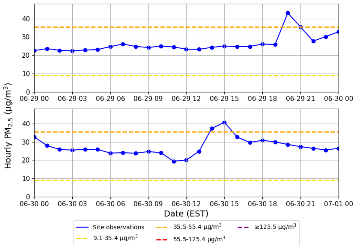
155 Figure E6. Hourly PM 2.5 concentrations at the Augusta site on June 29 and 30, 2023. The solid lines with dots show observations, and the dashed lines show AQI tiers adjusted for the 2024 PM 2.5 NAAQS.
