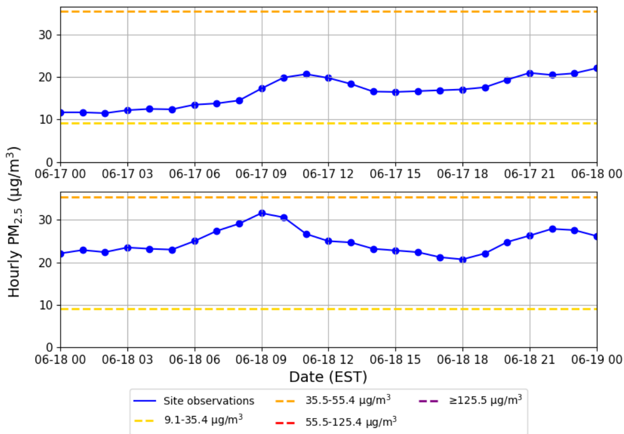
145 Figure E4. Hourly PM 2.5 concentrations at the Augusta site on June 17 and 18, 2023. The solid lines with dots show observations, and the dashed lines show AQI tiers adjusted for the 2024 PM 2.5 NAAQS.
