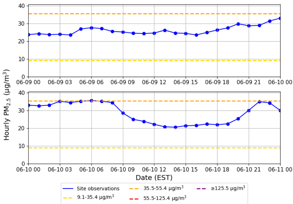
140 Figure E3. Hourly PM 2.5 concentrations at the Augusta site on June 9 and 10, 2023. The solid lines with dots show observations, and the dashed lines show AQI tiers adjusted for the 2024 PM 2.5 NAAQS.
