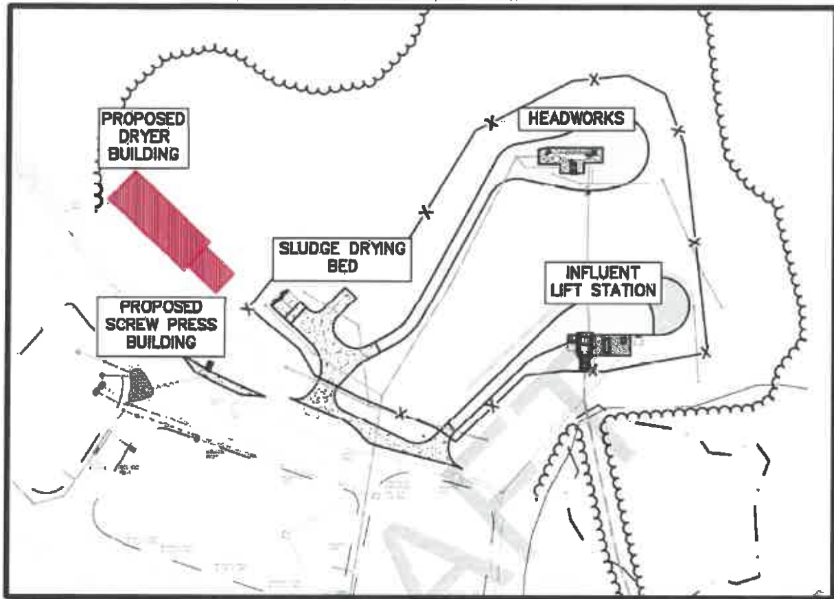
Figure 4: Conceptual Site Plan – Shoal Creek WWTP
