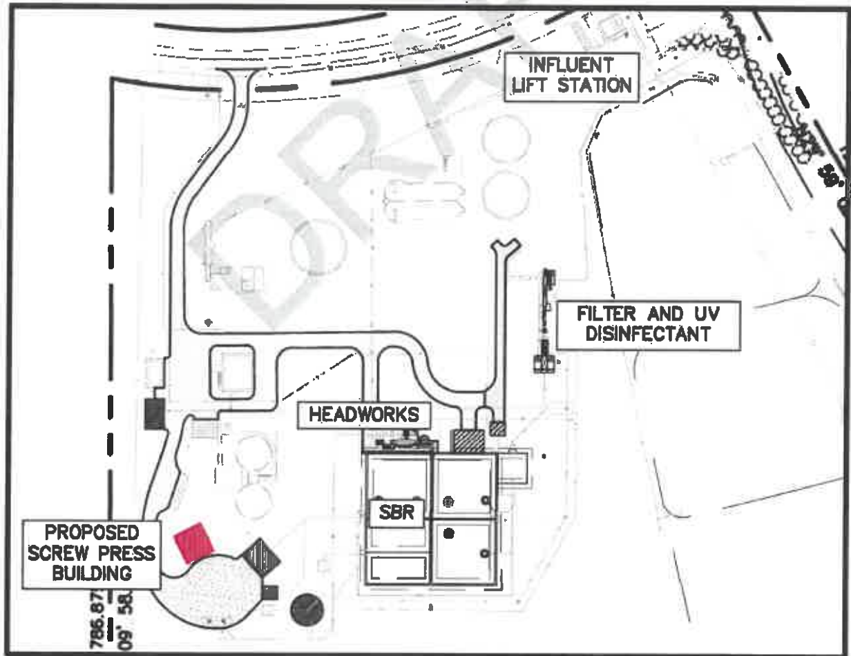
Figure 3: Conceptual Site Plan – Potato Creek WPCP
