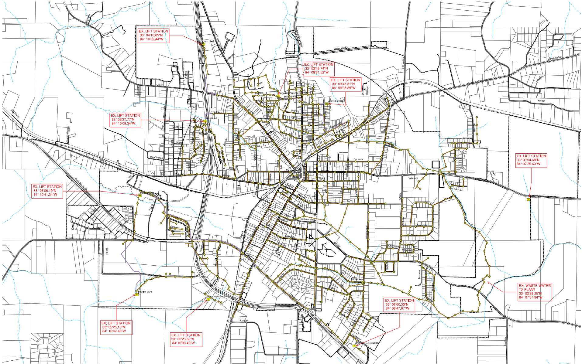
EXISTING SEWER SYSTEM MAP CITY OF BARNESVILLE
