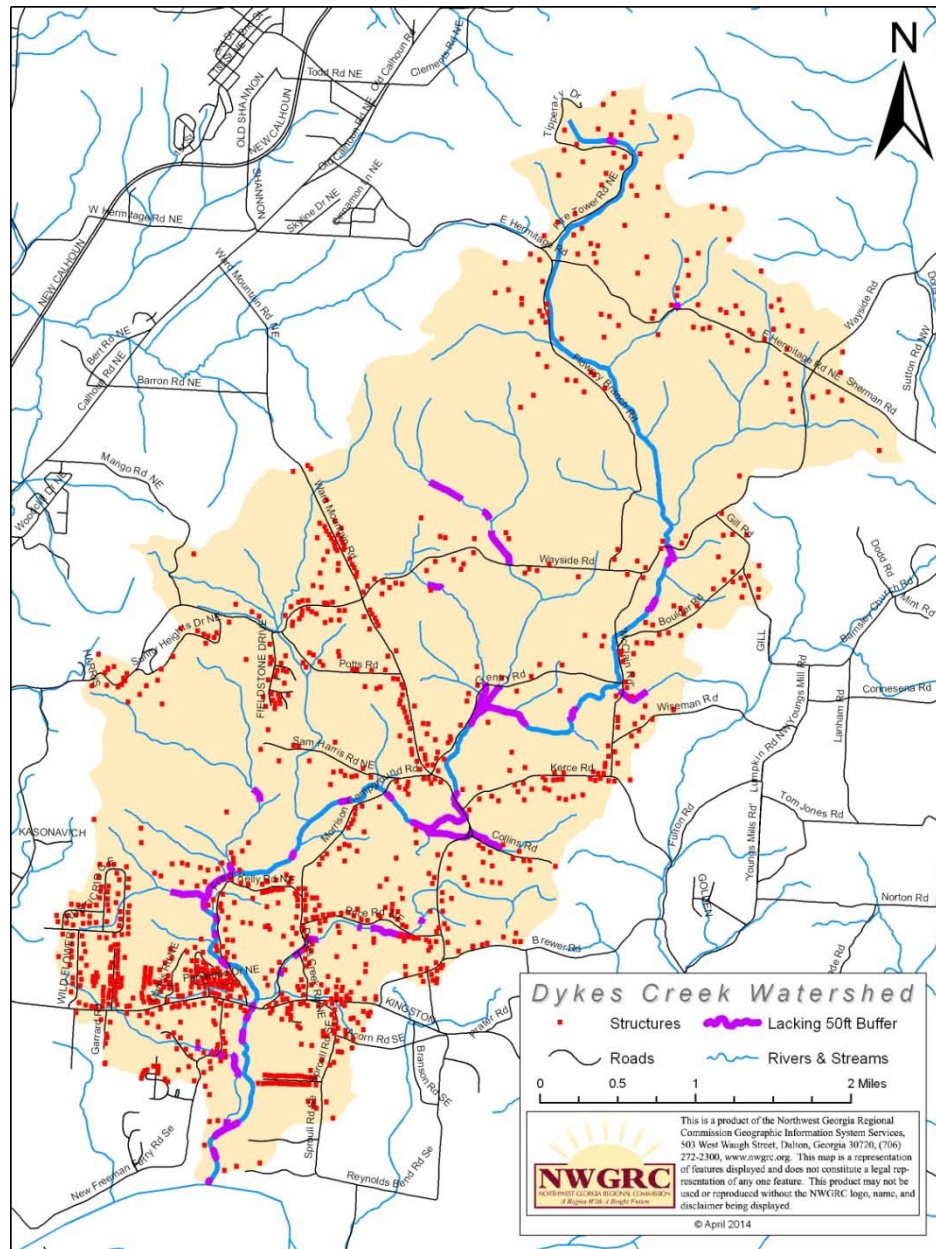
Figure 3.8. Map of insufficient 50 foot riparian buffers and total residential/business structures expected to have septic systems in the watershed.
