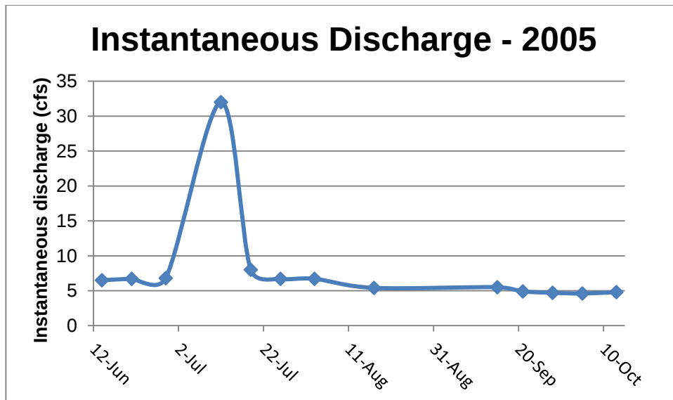
Figure 2.2 A display of the instantaneous discharge (flow) in Dykes Creek at Kingston Highway (SR 293) during summer and fall of 2005. Source: USGS
