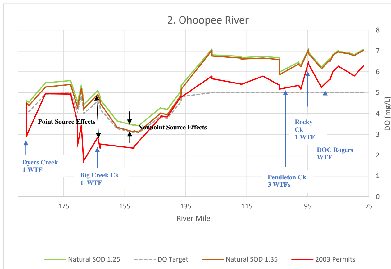
Figure 4-3. Natural, DO Target, Nonpoint Source, and Critical 2003 Permitted Oohoopee River Model Results.
