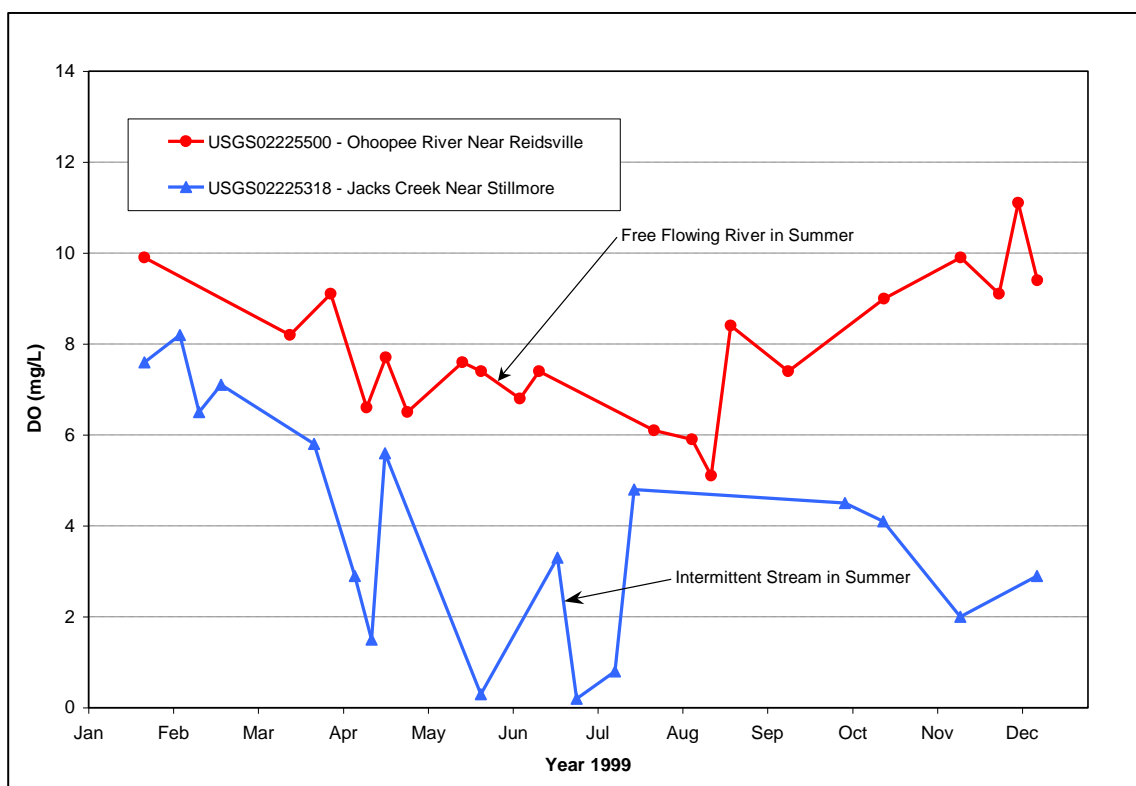
Figure 2-1. Comparison of Dissolved Oxygen Data at Two Oohopee River Basin Locations.
