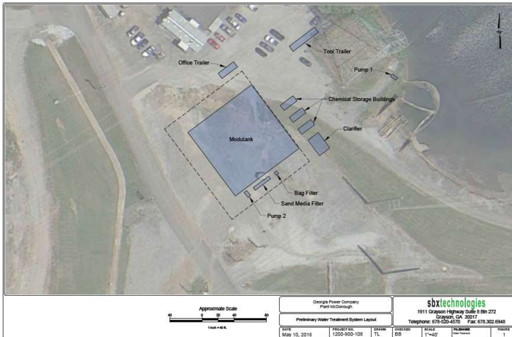
FIGURE 1 Treatment System Layout
