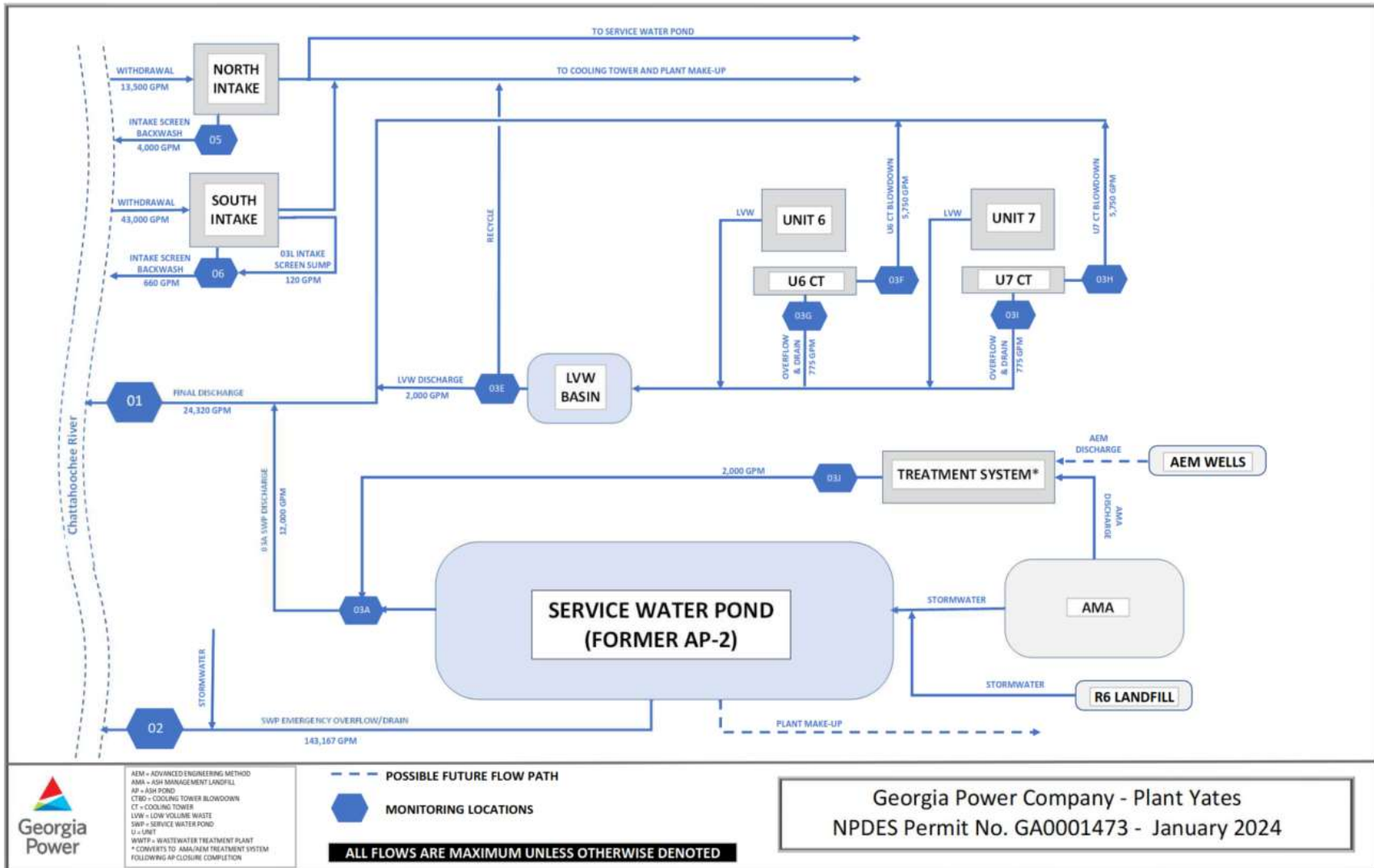
Figure 2C (Current Configuration)
