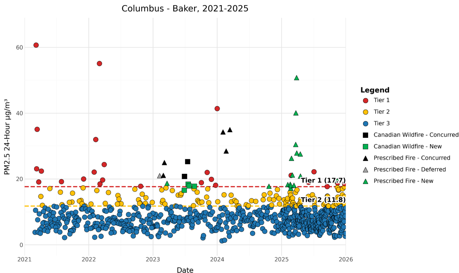
Figure 1. 24-hour PM 2.5 concentrations for 2021-2025 at the Columbus-Baker site. Days not submitted for exceptional events are demarcated by color with Tier 1 in red, Tier 2 in yellow, and Tier 3 in blue. Wildfire exceptional events are shown in squares, with black squares as concurred events and green squares as new events. Prescribed fire exceptional events are shown in triangles, with black triangles as concurred events, gray triangles as deferred events, and green triangles as new events.
