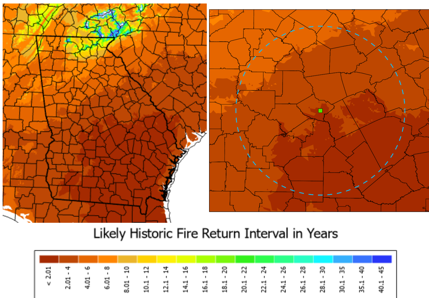
Figure 3. Natural fire return interval map for Georgia (left) and Macon (right). The Macon-Allied site is depicted with a green square, and the dashed line indicates a 100 km buffer around the Macon-Allied site.
