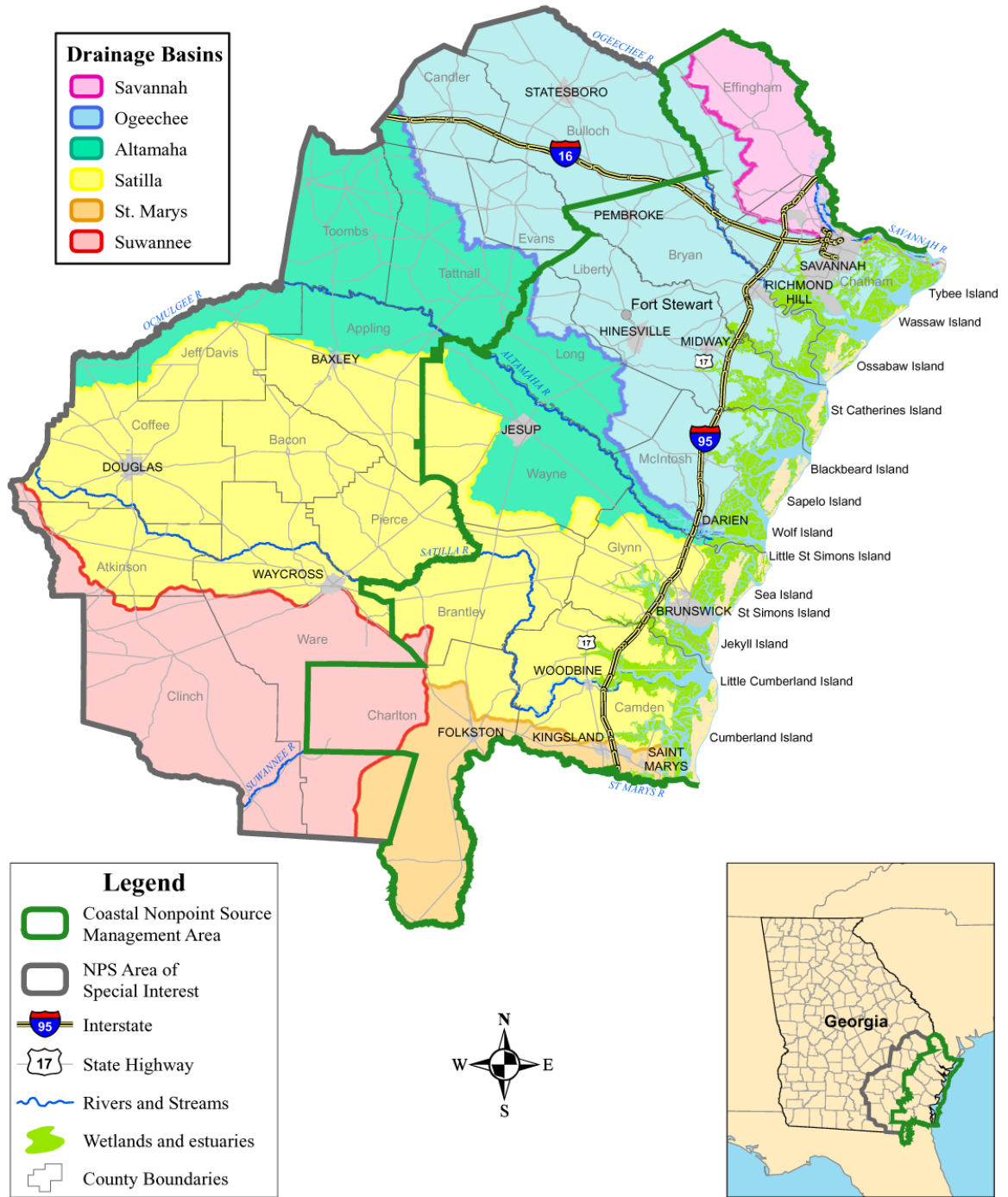
Figure 3. The Coastal Nonpoint Source Management Area
