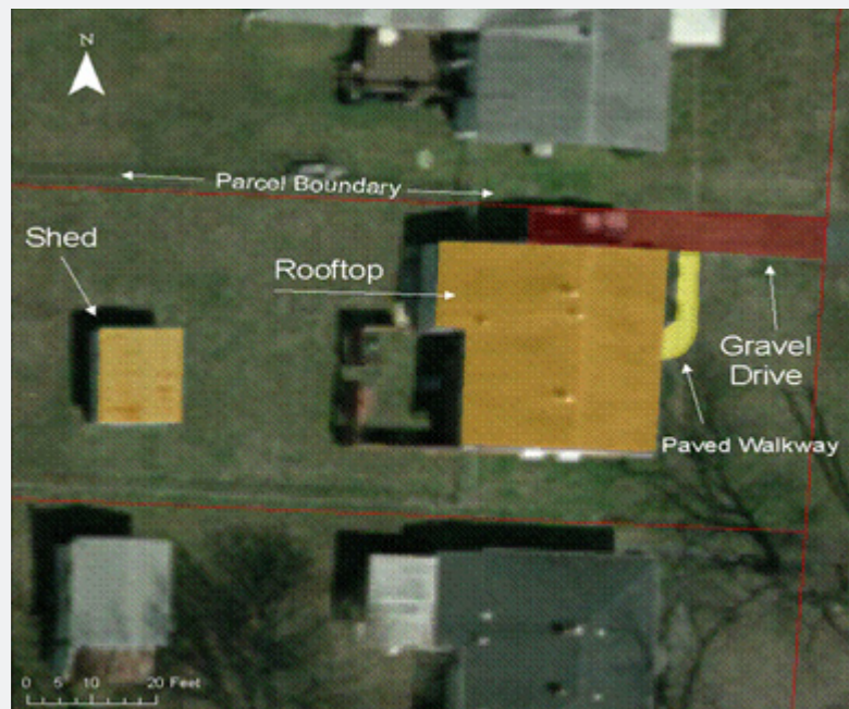
Figure CS-4. Sample Digitized Parcel Showing Rooftop and Paved Impervious Surface Footprints.
