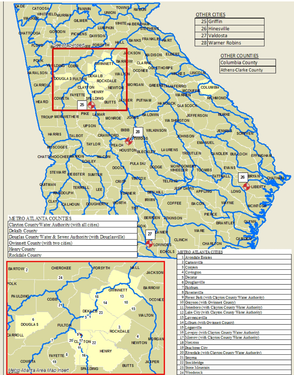
Figure 2. Locations with Stormwater Utilities in Georgia
