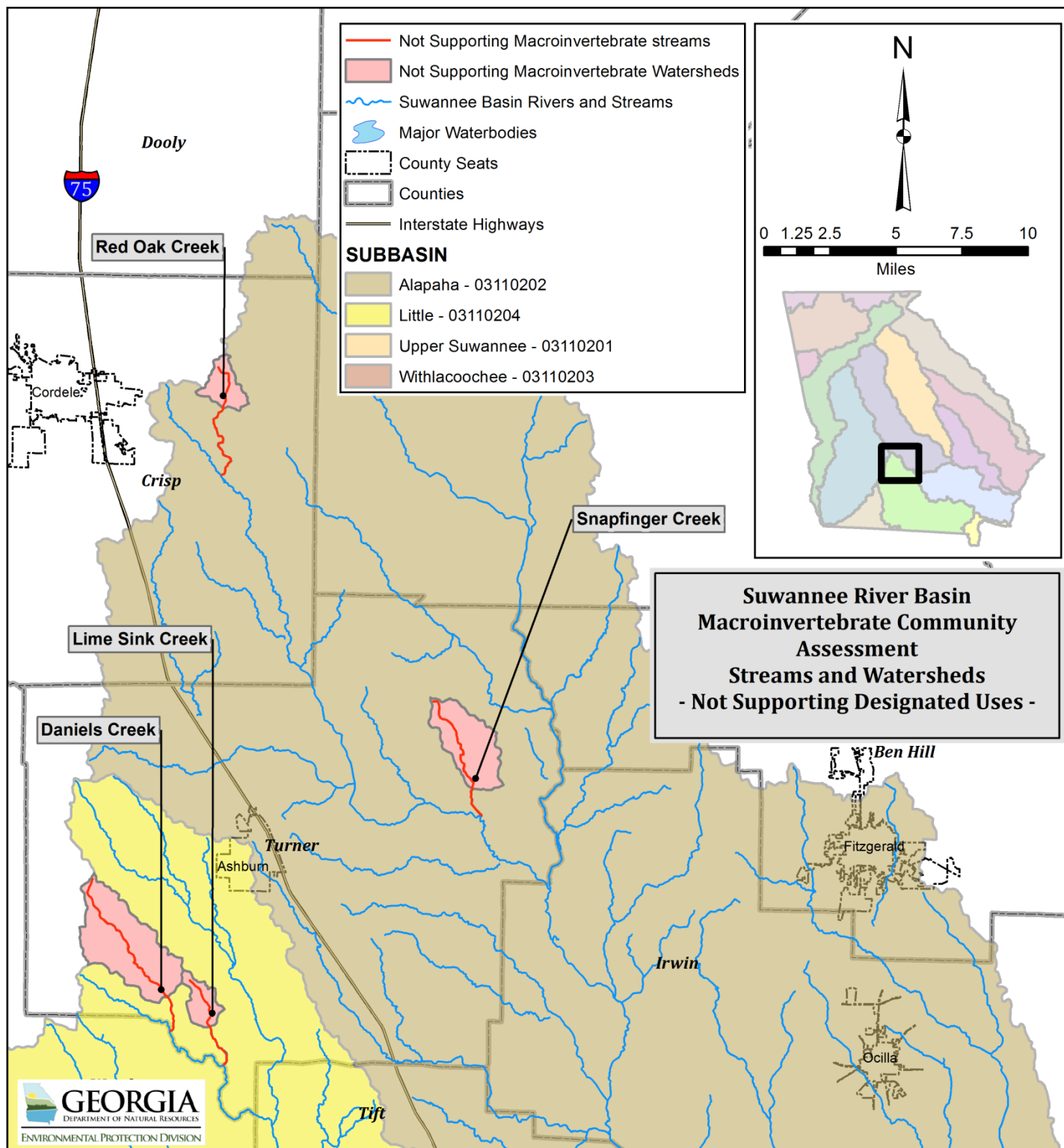
Figure 3. Macroinvertebrate Community Not Supporting Stream Segments and their Associated Watersheds - Upper portion of Suwannee River Basin
