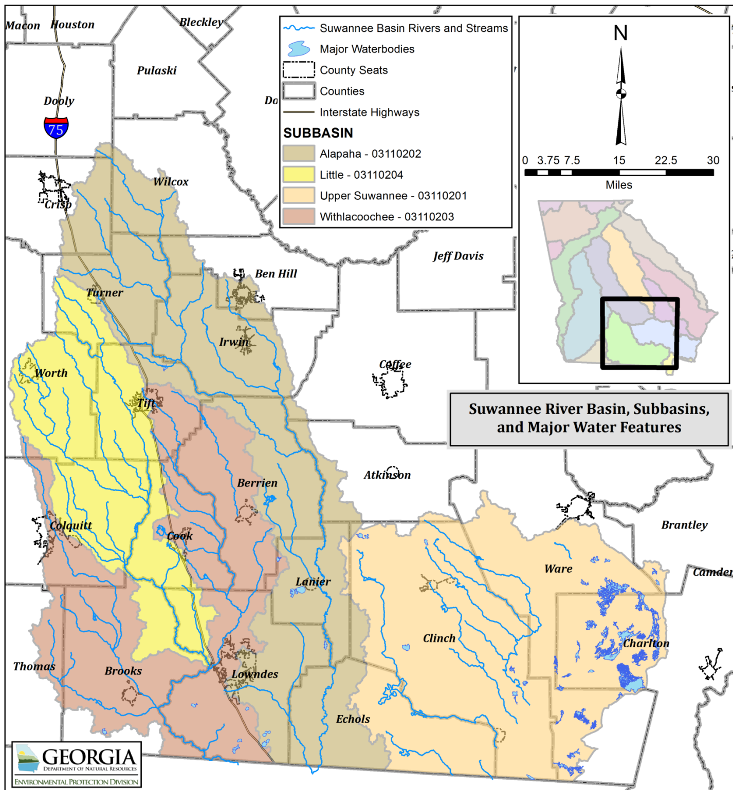
Figure 2: Suwannee River Basin, Subbasins, and Major Water Features
