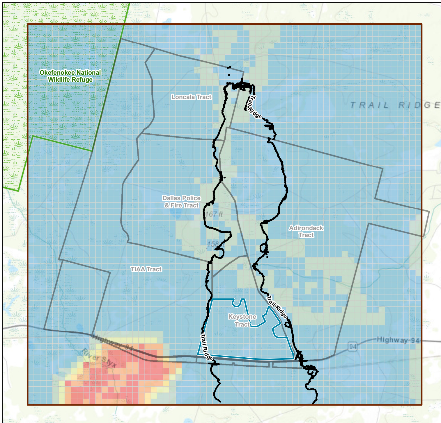
Figure 28 Calibrated Horizontal Hydraulic Conductivity in Silty Clayey Sand Unit (HSU 3)
