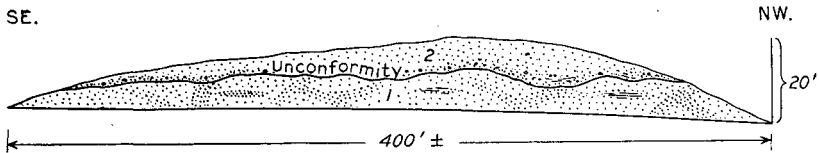
Fig. 13.—Section in cut of Central of Georgia Railway, six miles south-east of Eufaula, Ala., in Quitman County, Ga.
