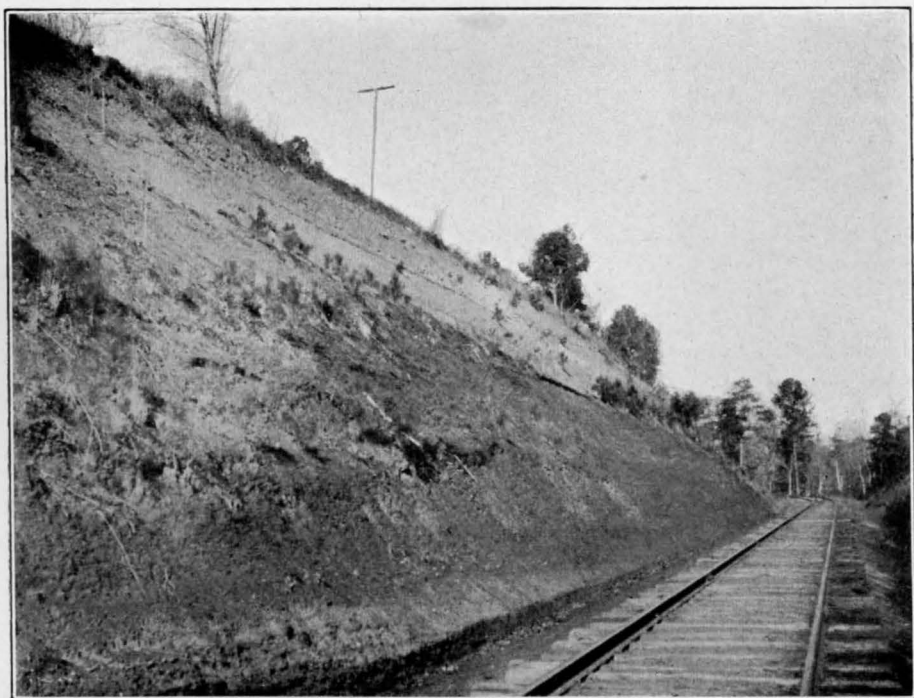
B. CUT OF ATLANTA, BIRMINGHAM & ATLANTIC RAILROAD, ONE AND ONE-EIGHTH MILES NORTH OF IDEAL, MACON COUNTY, GA., SHOWING MARINE SANDS AND CLAYS OF THE RIPLEY FORMATION.
