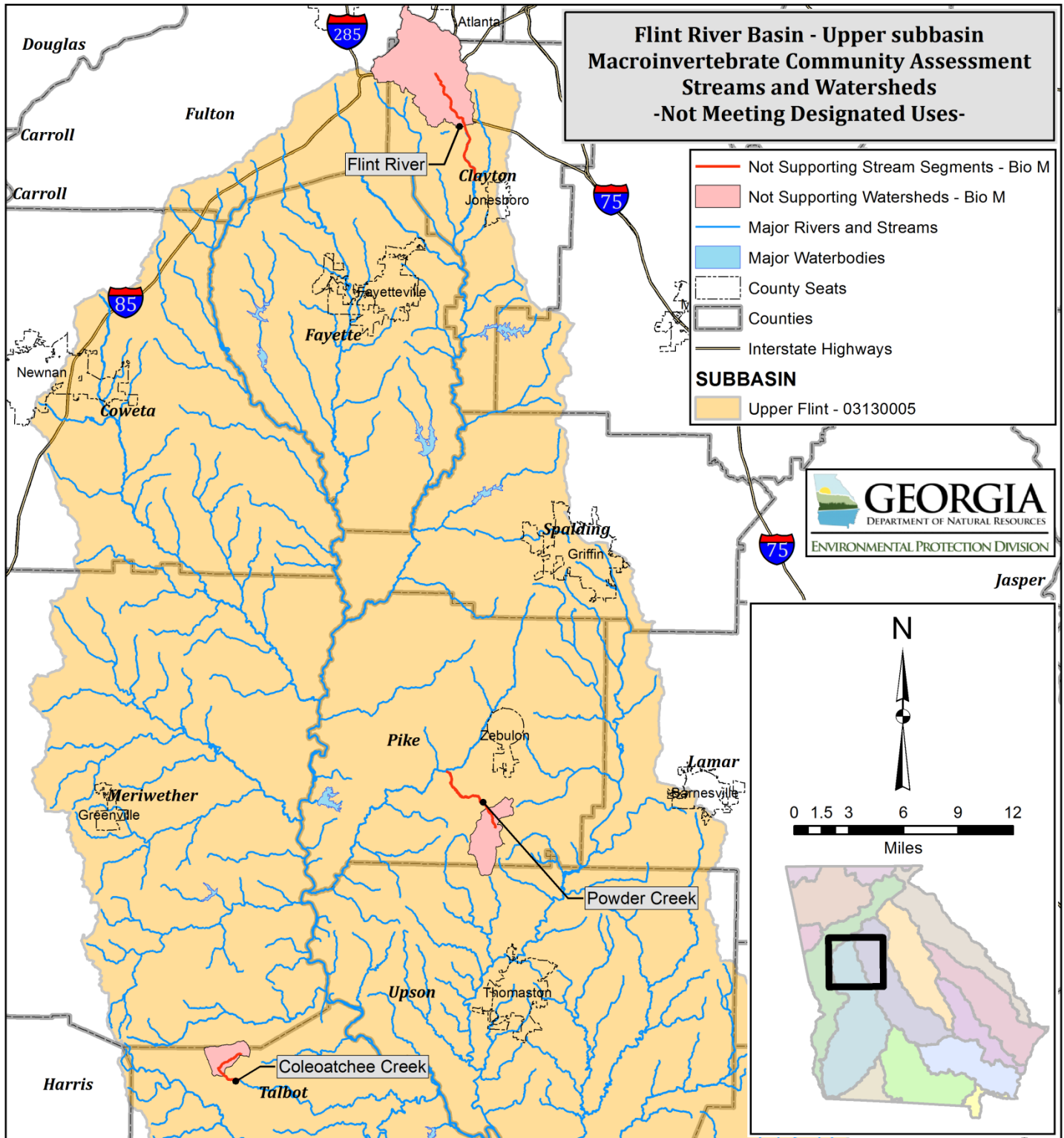
Figure 4. Macroinvertebrate Community Not Supporting Stream Segments and their Associated Watersheds - Upper Flint Subbasin
