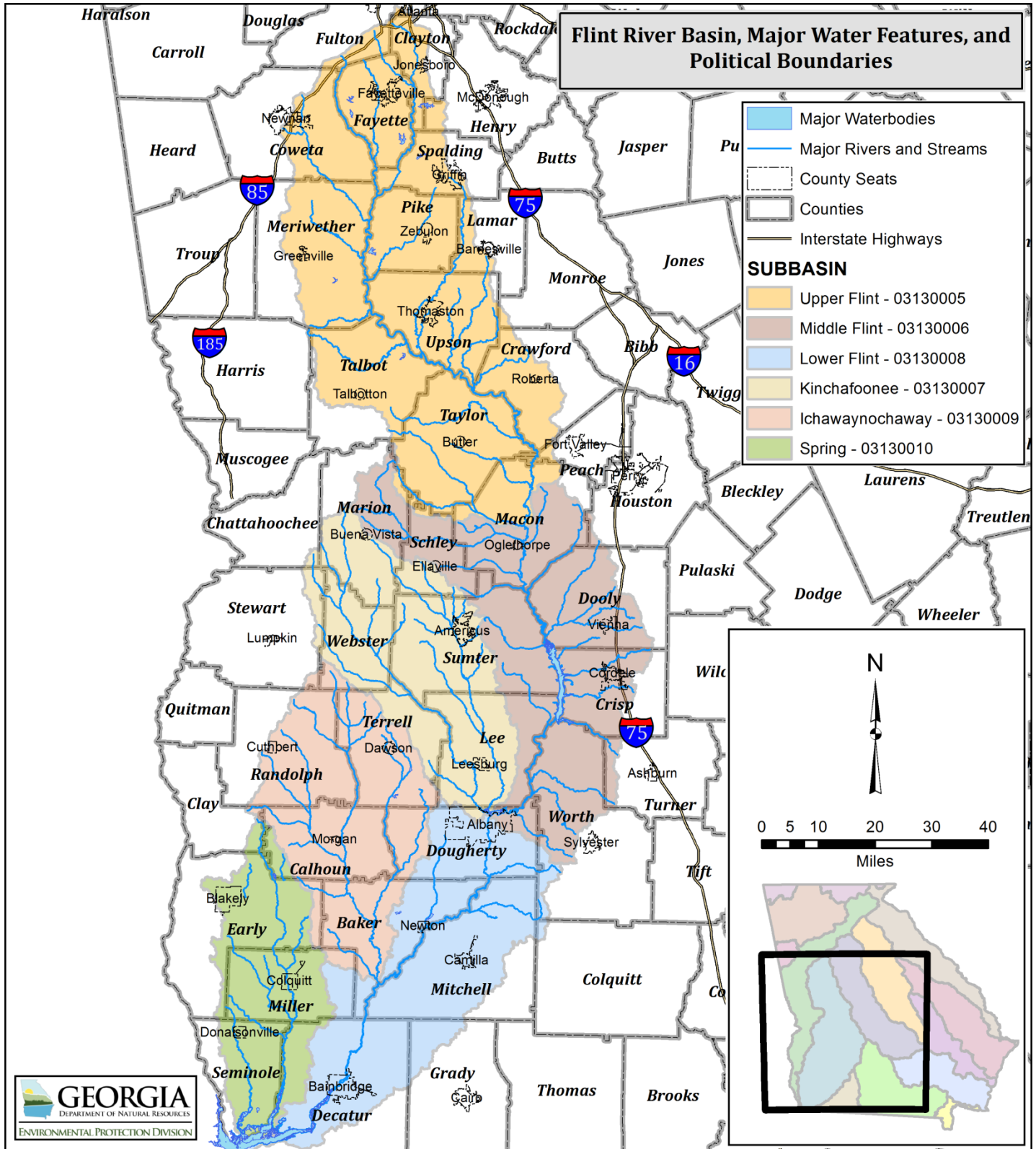
Figure 2. Flint River Basin, Subbasins, Major Water Features, and Political Boundaries
