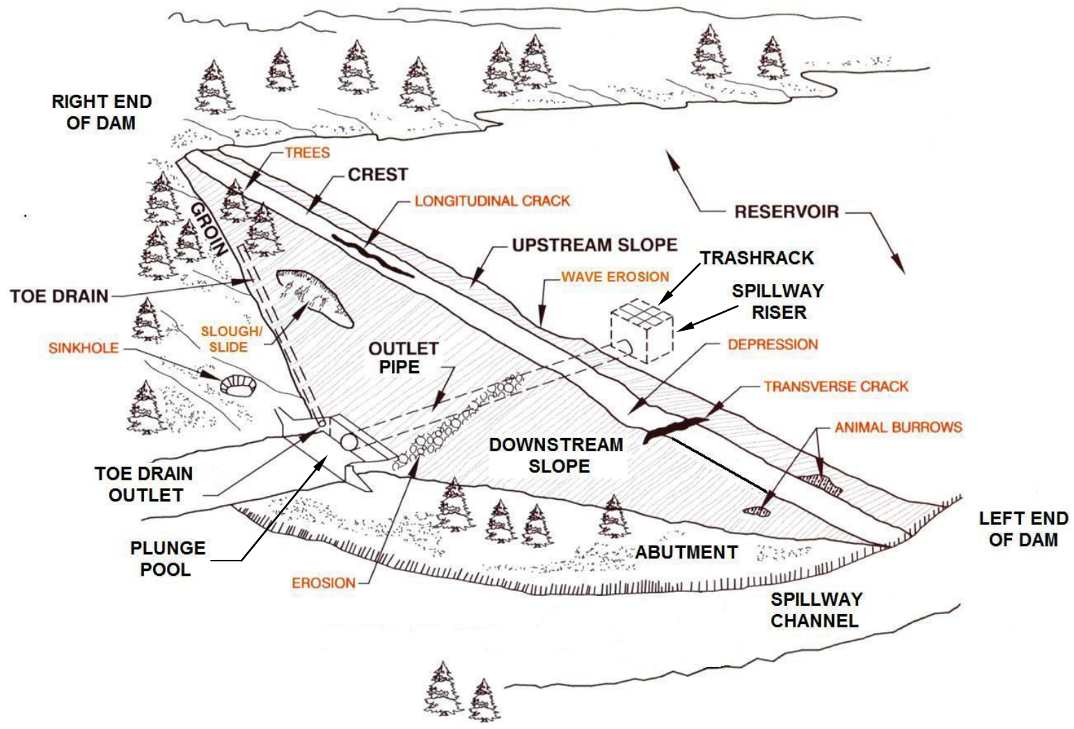
TYPICAL EMBANKMENT DAM (COMMON DEFICIENCIES NOTED IN ORANGE)
