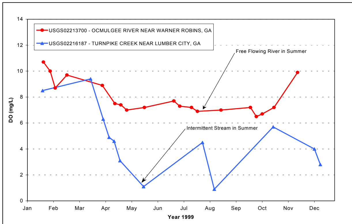
Figure 3-1. Comparison of Dissolved Oxygen Data at Two Ocmulgee River Basin Locations.
