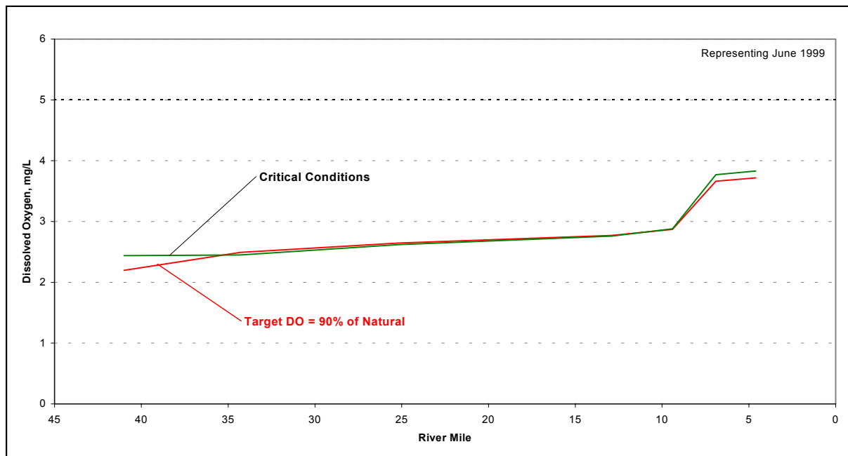
Figure 6-4. Critical Conditions and 90% of Natural Conditions for a Watershed without Point Sources (Turnpike Creek).
