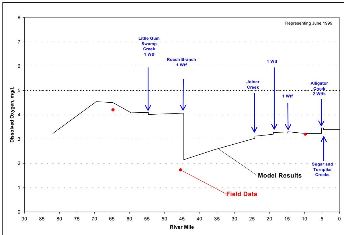
Figure 6-1. Dissolved Oxygen Calibration for the Little Ocmulgee River.
