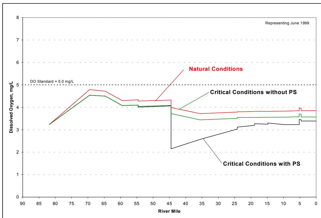
Figure 6-2. June 1999 Critical and Natural Conditions for the Little Ocmulgee River.
