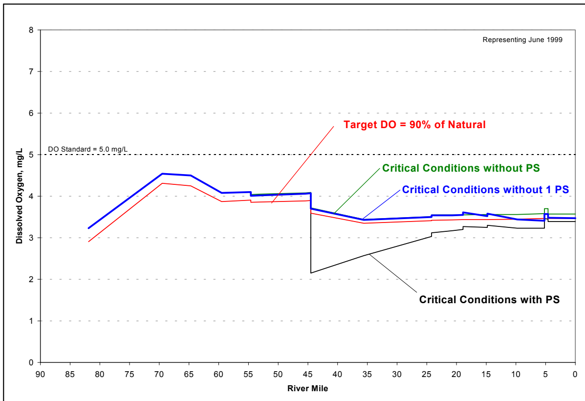
Figure 6-3. Critical Condition Scenarios and 90% of Natural Conditions of the Little Ocmulgee River Basin.
