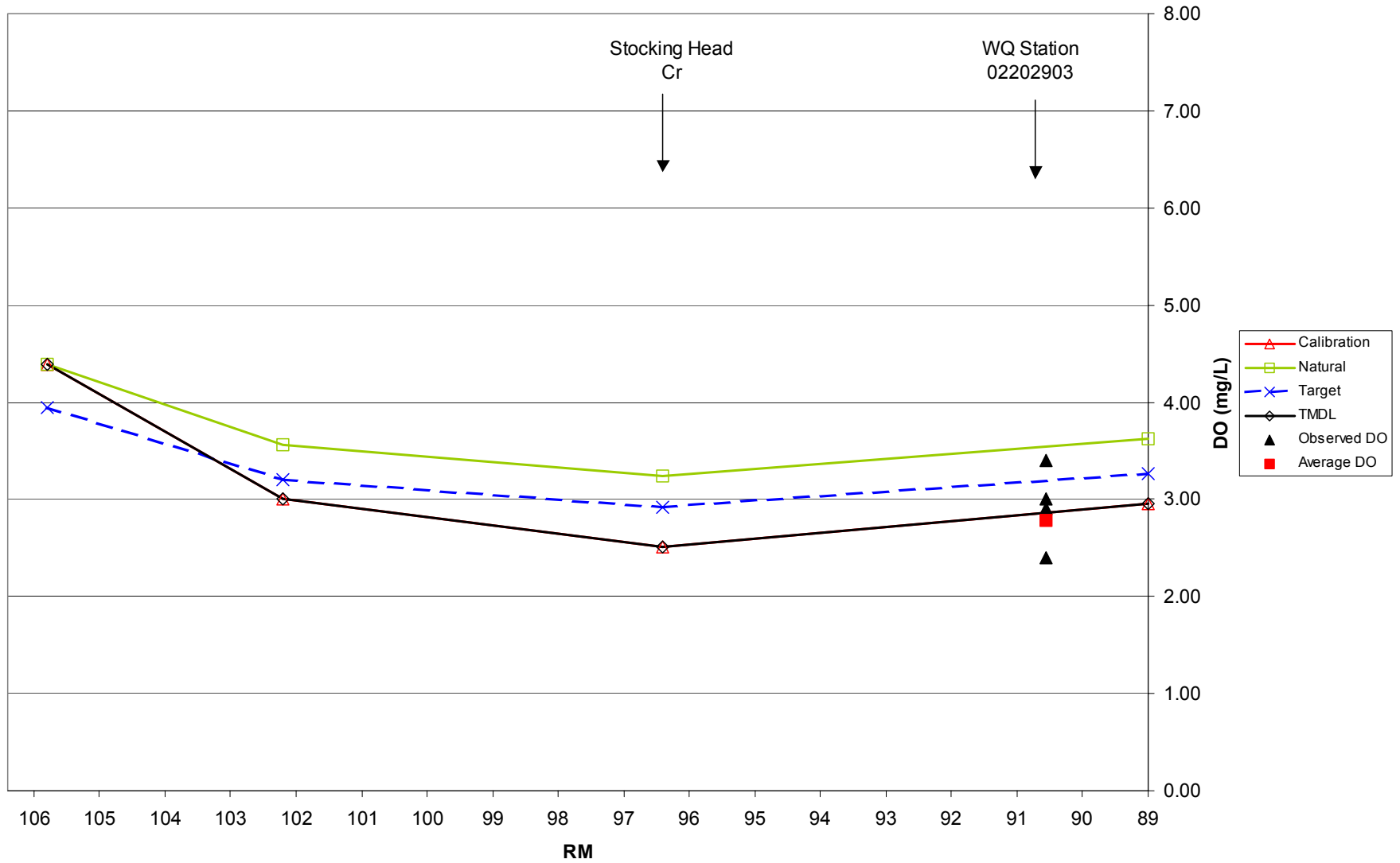
Figure C-2b DOSAG Model Results Fifteenmile Creek
