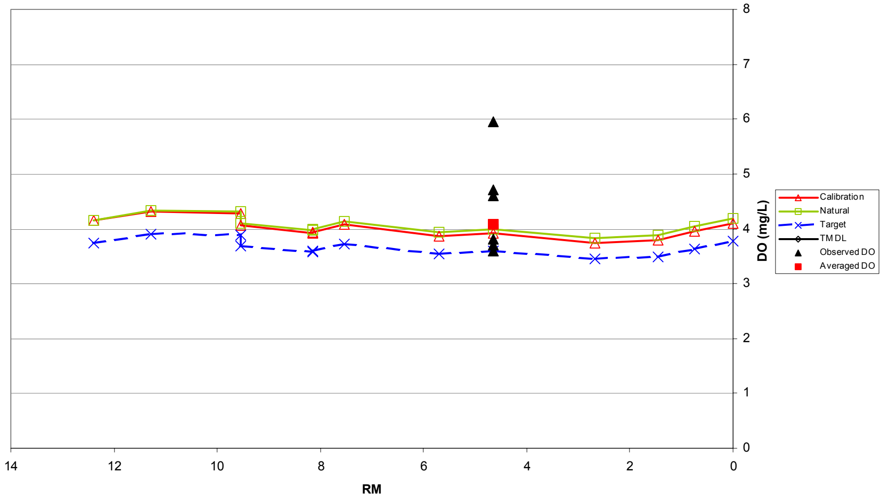
Figure C-9 DOSAG Model Results Peacock Creek
