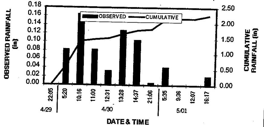
FIGURE 2: RAINFALL RECORD (UPPER CHATTOOGA RIVER TMDL PROJECT)
