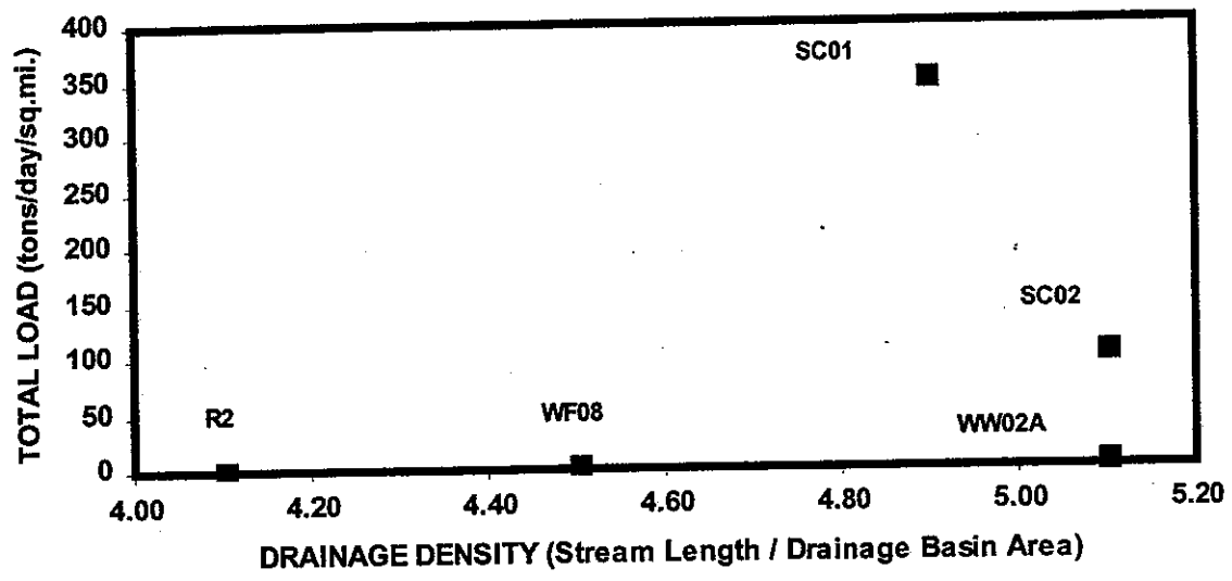
FIGURE 13: PEAK TOTAL SEDIMENT LOAD DURING STORM EVENT (Upper Chattooga River TMDL Project)
