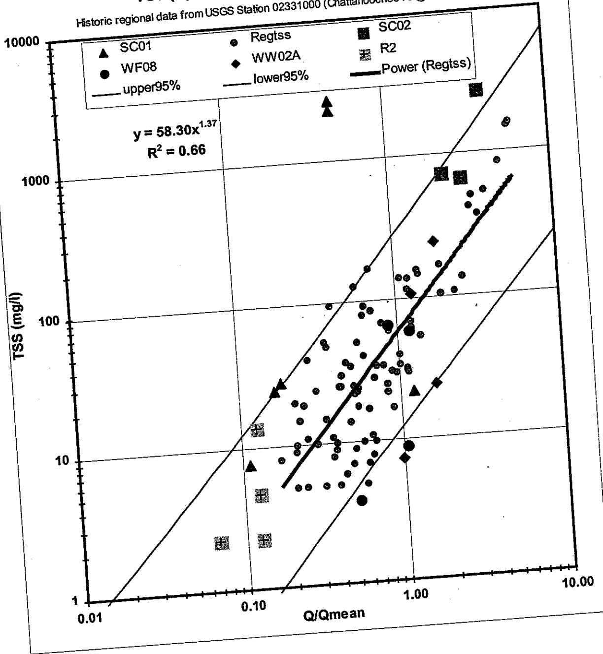
FIGURE 7 : OBSERVED TSS OVERLAYING HISTORIC REGIONAL TSS (Upper Chattooga River TMDL Project)
