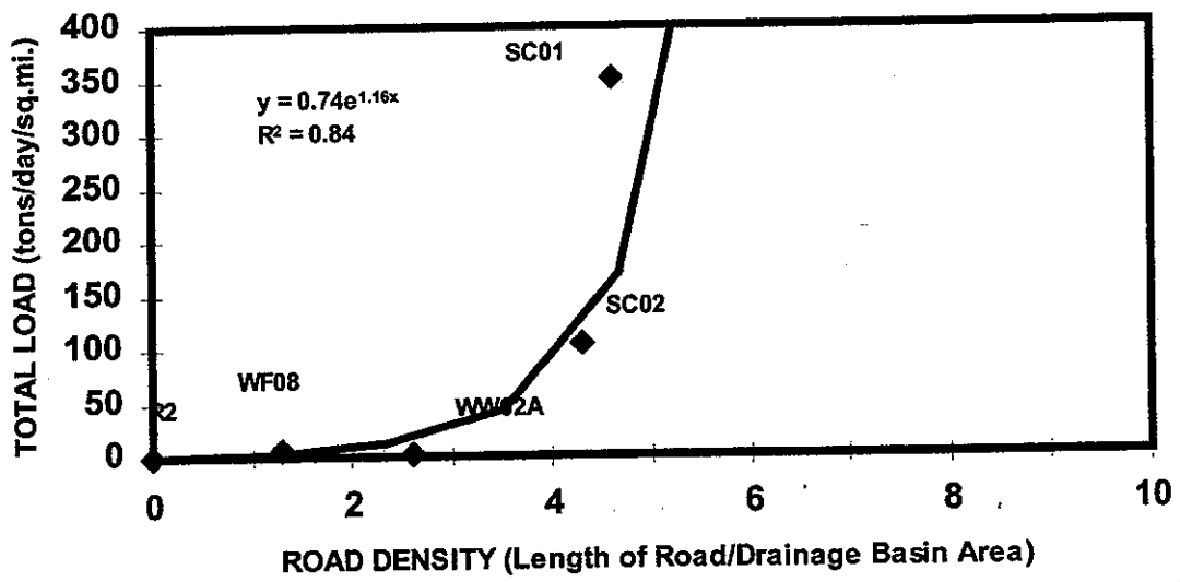
FIGURE 13: PEAK TOTAL SEDIMENT LOAD DURING STORM EVENT (Upper Chattooga River TMDL Project)
