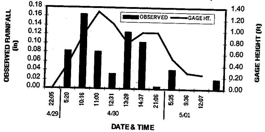
FIGURE 3: RAINFALL RECORD AND GAGE HEIGHT (UPPER CHATTOOGA RIVER TMDL PROJECT)
