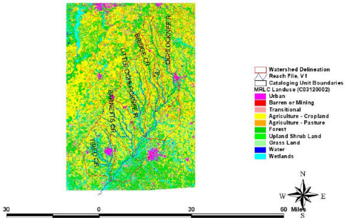
Figure 3 Ochlockonee Watershed Landuses
