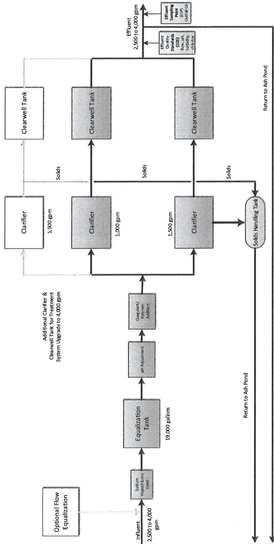
FIGURE 1 Plant Branch Treatment System Schematic with an option to upgrade from 2,500 gpm to 4,000 gpm
