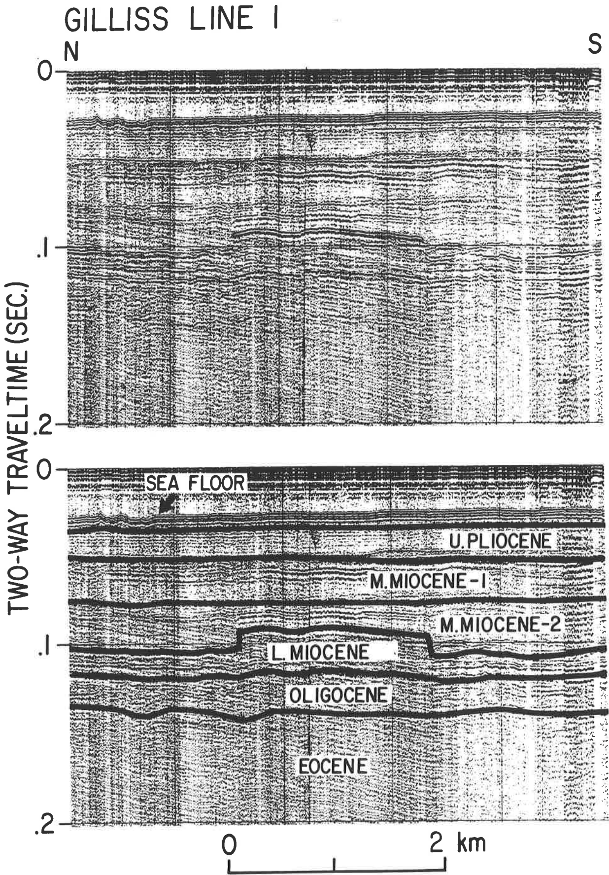
Figure 8. Part of GILLISS line 1 from the inner shelf off southern Georgia. This record shows an erosional remnant layer of strata preserved as an outlier. This type of discontinuous erosion of a resistant layer is characteristic of the top of lower Miocene strata (top of Burdigalian) and may be due to ravinement at the shore face.
