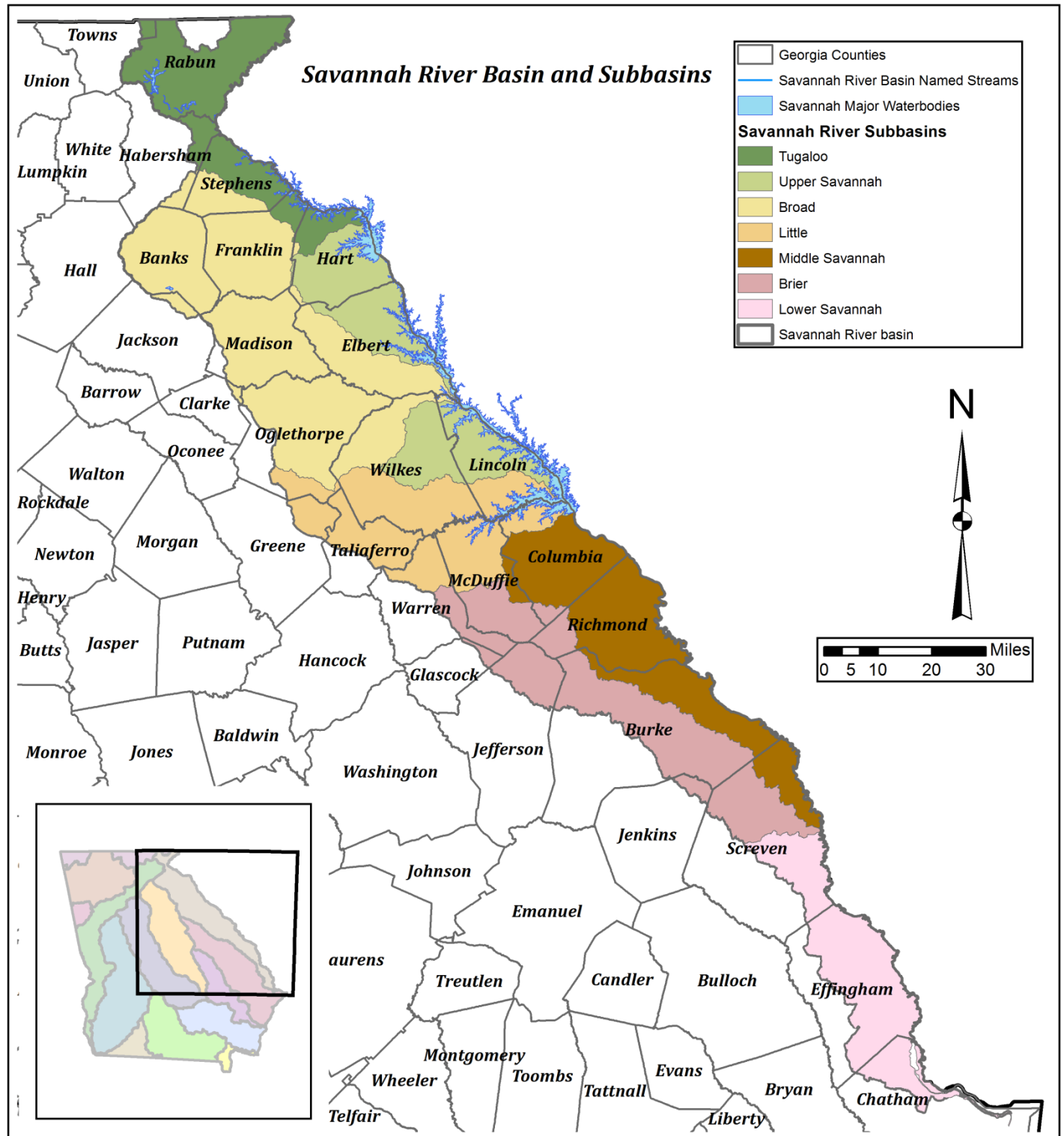
Figure 2: Savannah River Basin and Subbasins
