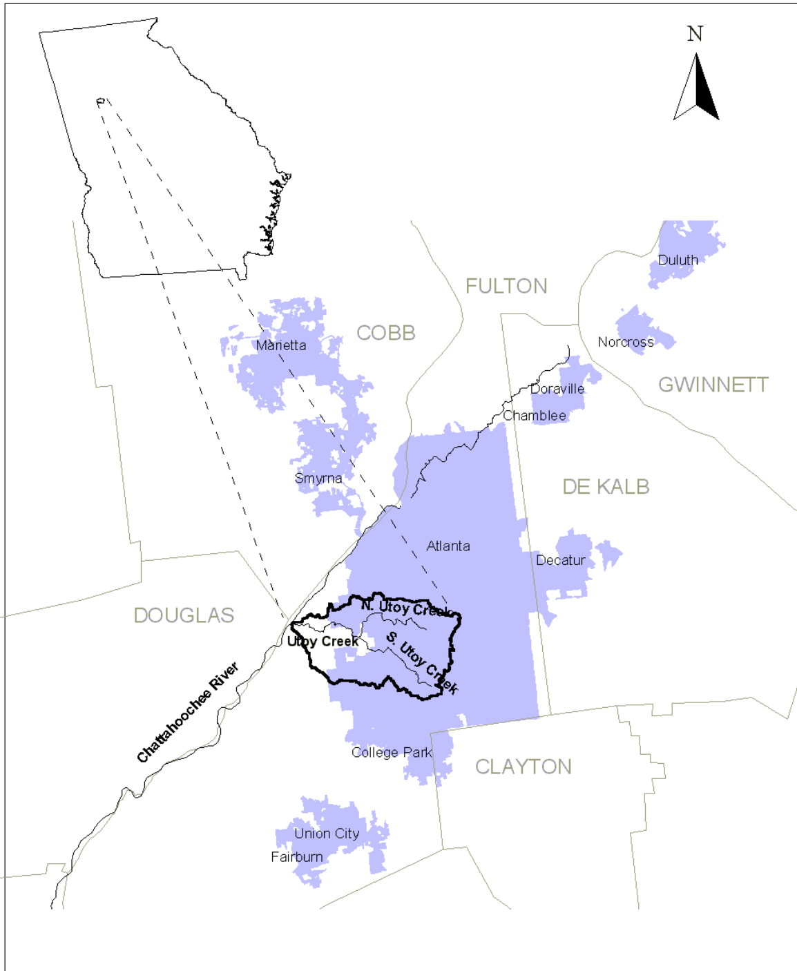
Figure 1. Utoy Creek Watershed
