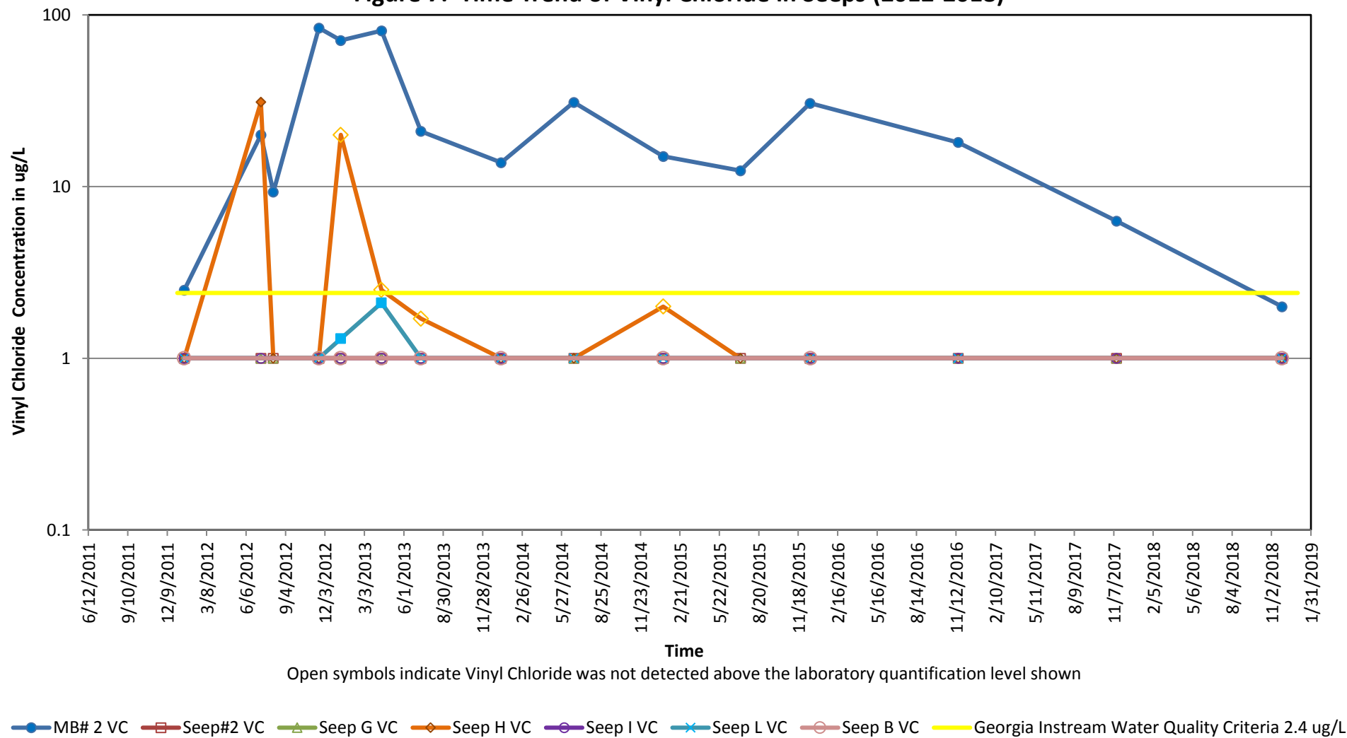
Figure 7: Time Trend of Vinyl Chloride in Seeps (2012-2018)
